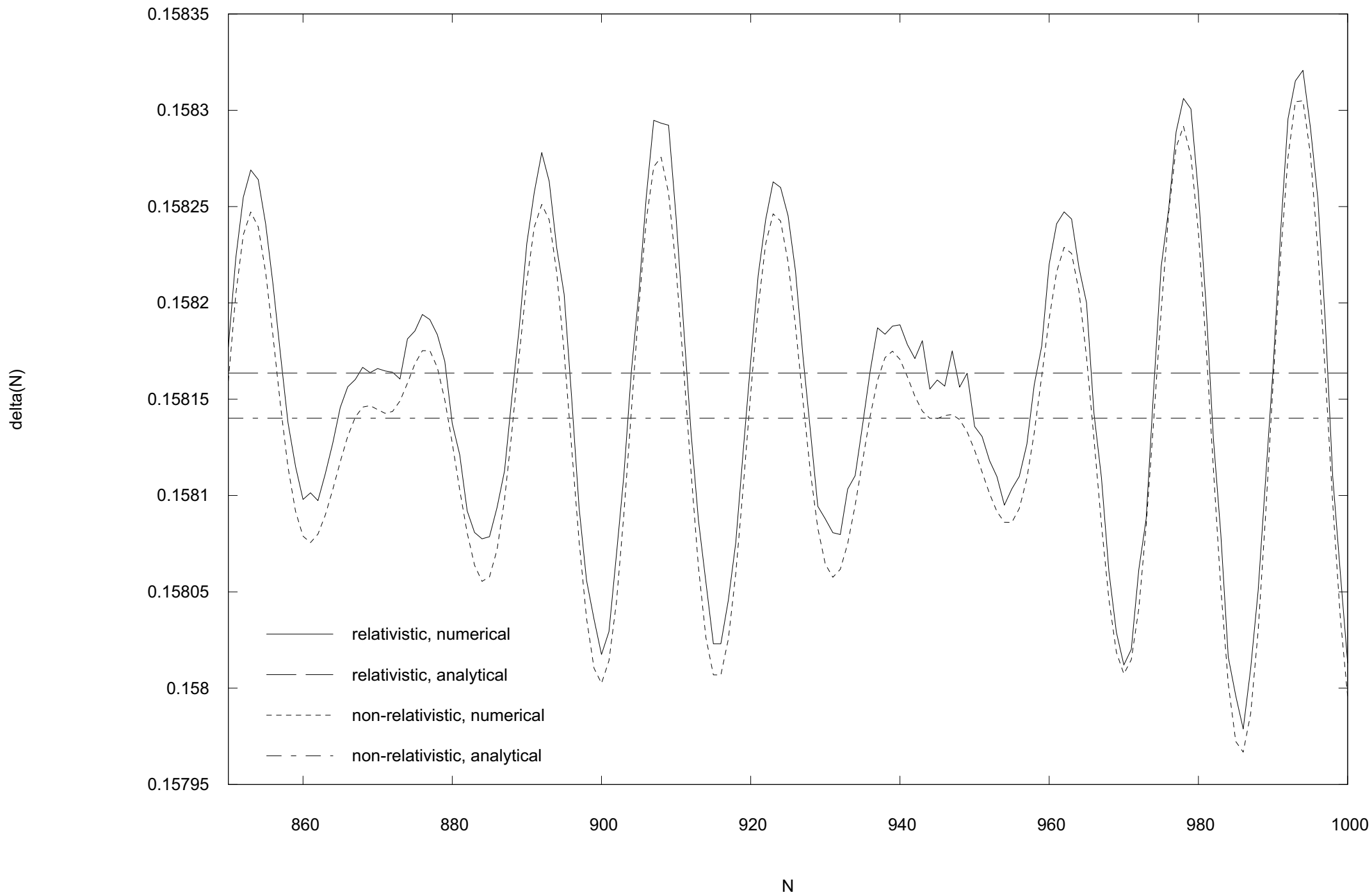
Comparison of relativistic and non-relativistic results, square-well, laguerre basis
